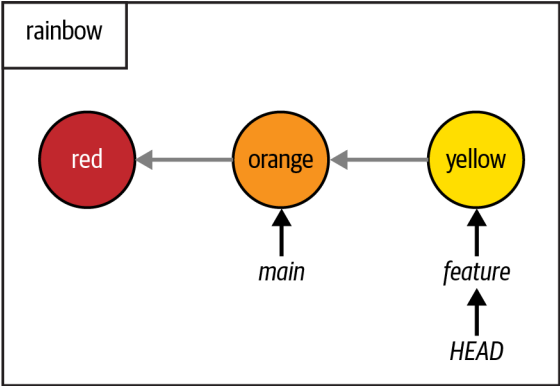
FIGURE C-6 An example of a Repository Diagram with one local repository, representing the state of the Rainbow project at the end of Chapter 4
