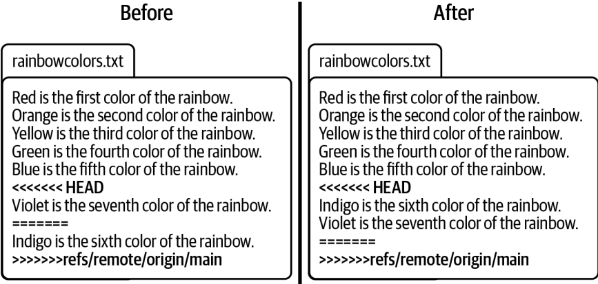
FIGURE 10-2 The rainbowcolors.txt file before and after your friend decides what to keep and edits the content
