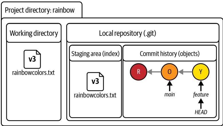
FIGURE C-5 An example of a Git Diagram with representations of the working directory, staging area, commit history, and local repository, showing the state of the Rainbow project at the start of Chapter 5
