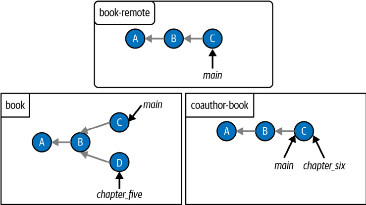
FIGURE 11-4 The Book project after I pull the changes from the remote main branch
