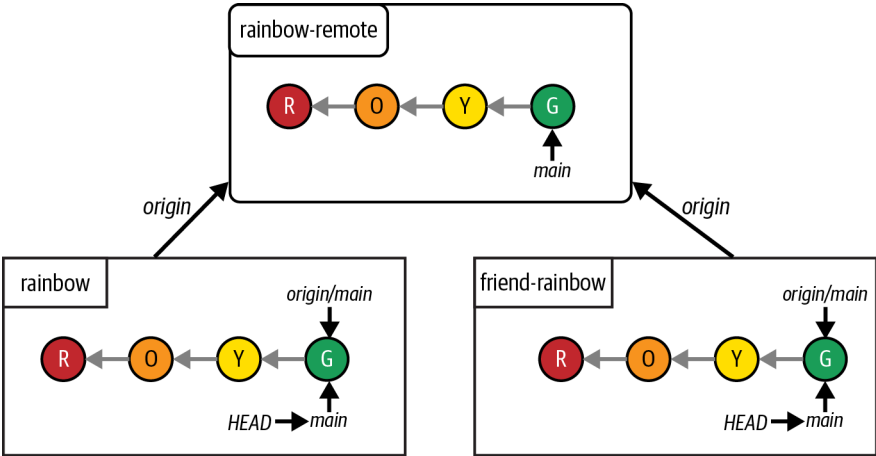
FIGURE C-7 An example of a Repository Diagram with two local repositories and one remote repository, representing the state of the Rainbow project at the end of Chapter 8
